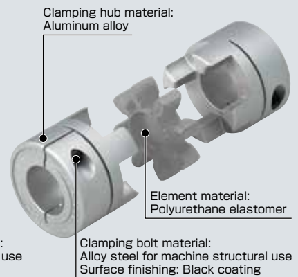
Clamp Type
